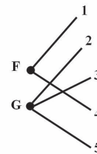
Figure 3: An example of juxtaposition \otimes_{\mathcal{I}}(F, G) , where \mathcal{I} = \{\{1, 4\}, \{2, 3, 5\}\} .
