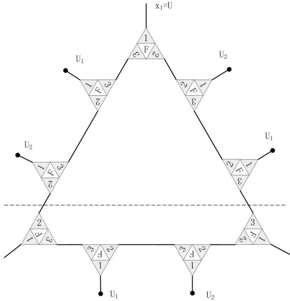
Figure 4: Gadget to realize a symmetric ternary function.
